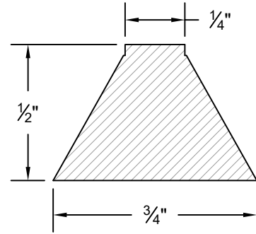
#2 3/4" RAISED MUNTIN
