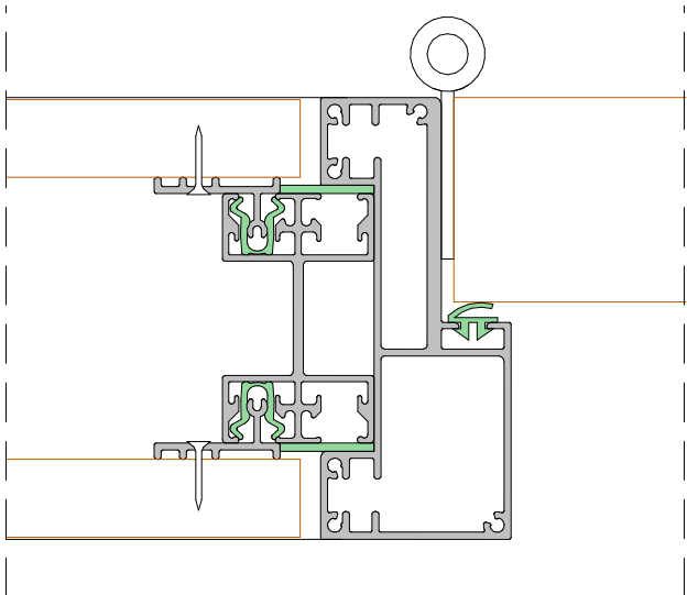
PA 100 OPAQUE CONNECTION TO 108MM (4 1/4") DOOR FRAME FOR 50MM (2") DOORS
