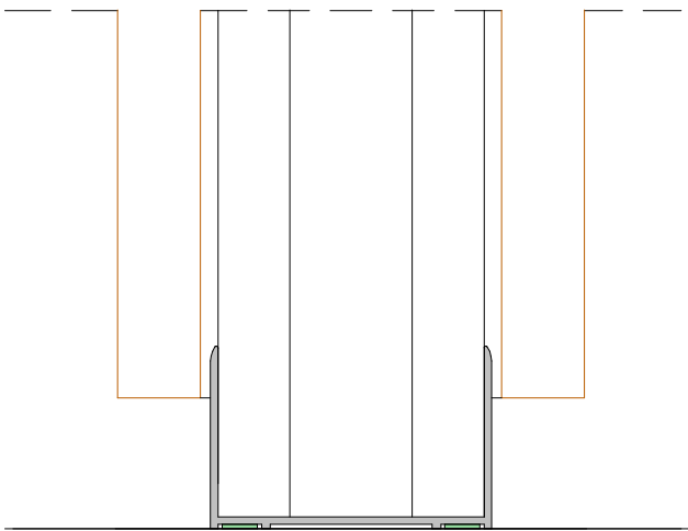
PA 100 OPAQUE FLOOR DETAIL
