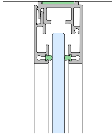
CEILING DETAIL
