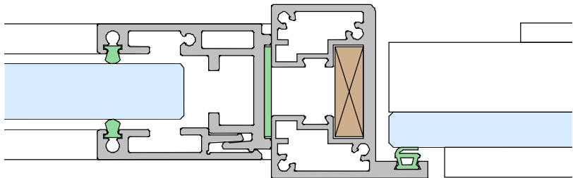
CONNECTION OF GLASS SLIM WITH 16MM ( \frac{5}{8} " ) GLASS TO GLASS SLIM DOOR FRAME
