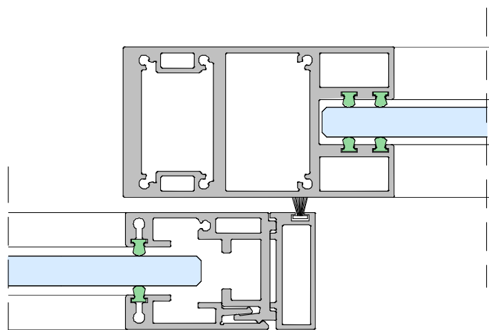
WOD GLASS SLIM DETAIL
