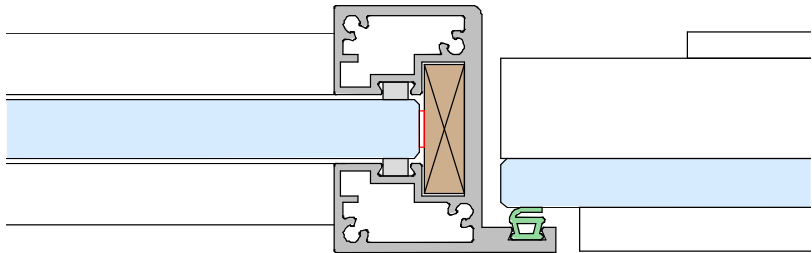
CONNECTION OF GLASS SLIM WITH 10 OR 12MM ( \frac{3}{8} " OR \frac{1}{2} " ) GLASS TO GLASS SLIM DOOR FRAME
