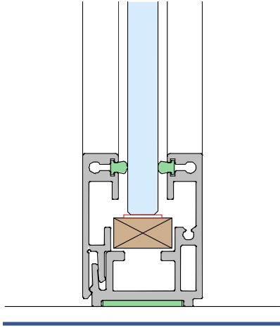
FLOOR DETAIL
