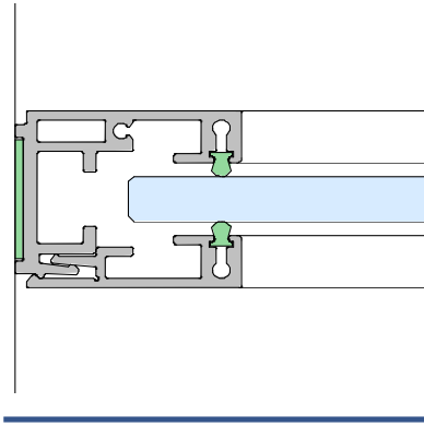
WALL DETAIL
